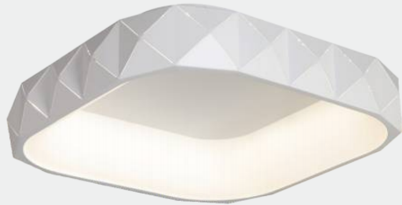
● CEILING DH-7123W-M 410*410*110mm DH-7123W-L 510*510*110mm
